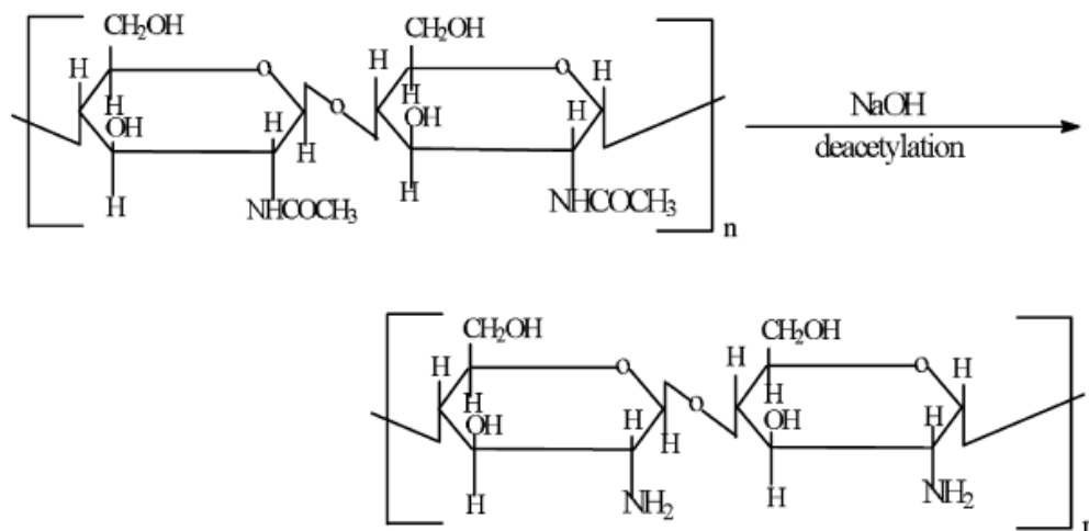
Scheme 2. Chitin deacetylation
