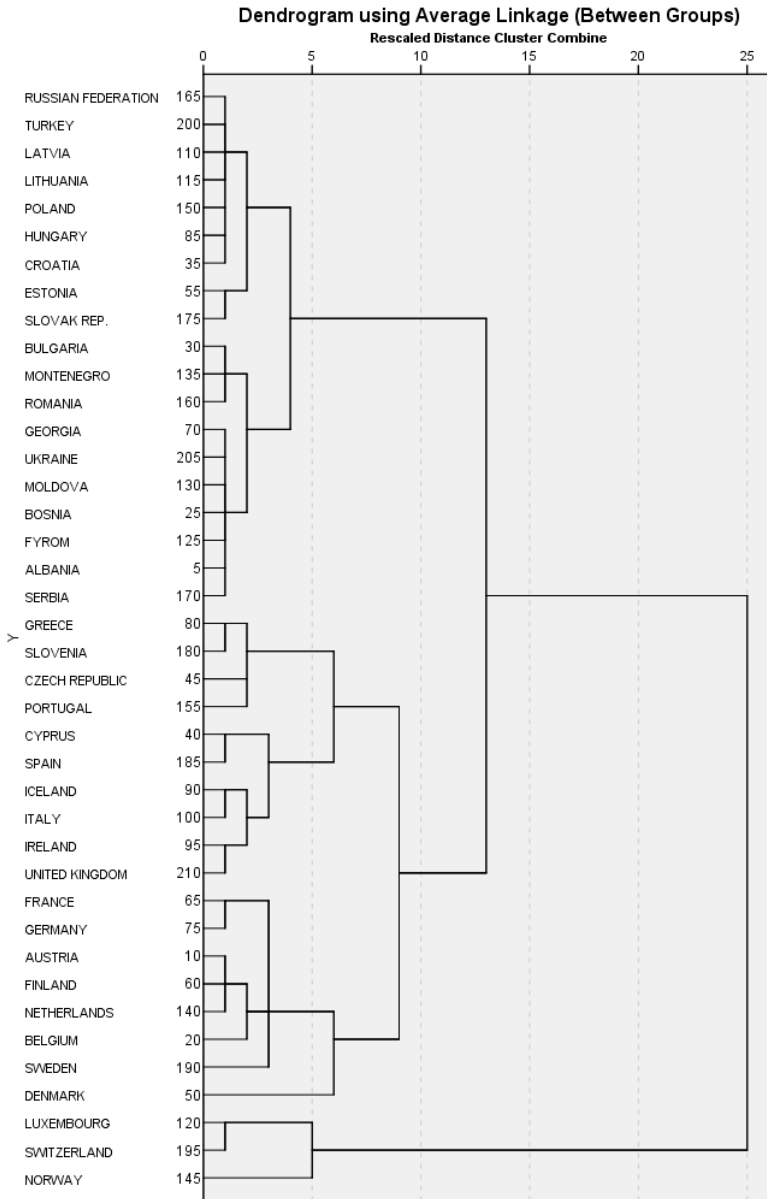
Figure 41 Dendrogram using average linkage between groups
