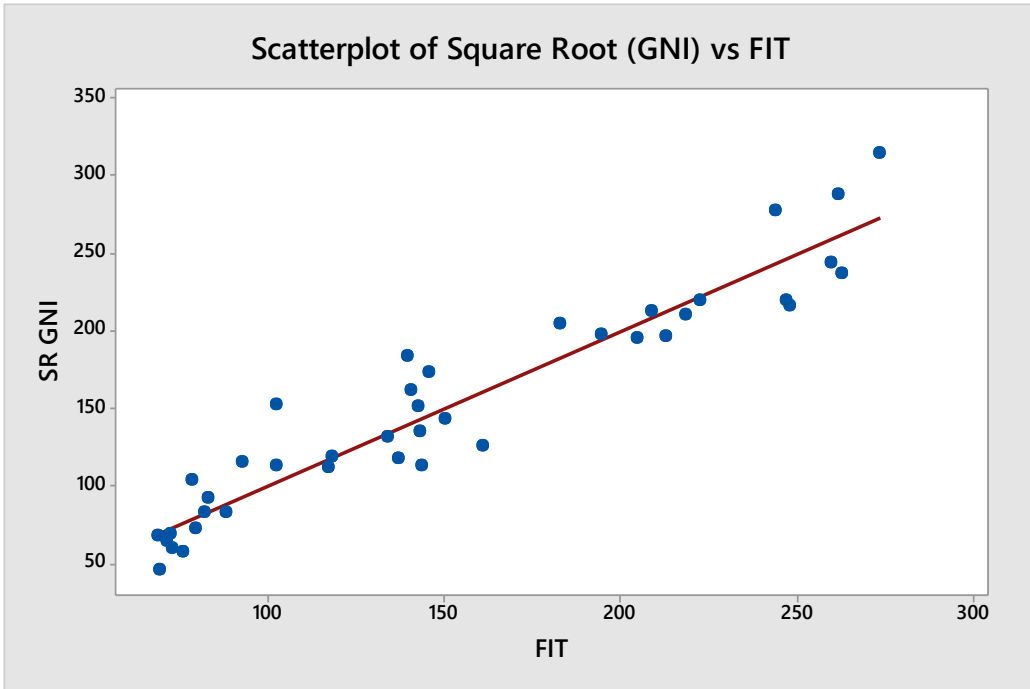
Figure 40 Observation values versus fitted values. All points are in a well-defined strip which indicate the constancy of the variations.
