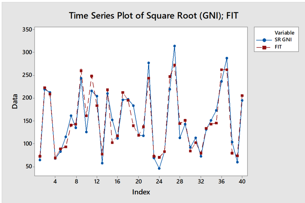
Figure 39 Observation values and fitted values versus order (alphabetical order of the countries). The fitted values are very close to the observations.
